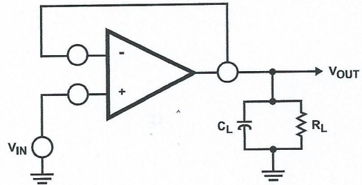
FIGURE 2. TRANSIENT RESPONSE TEST CIRCUIT FOR ALL TYPES
